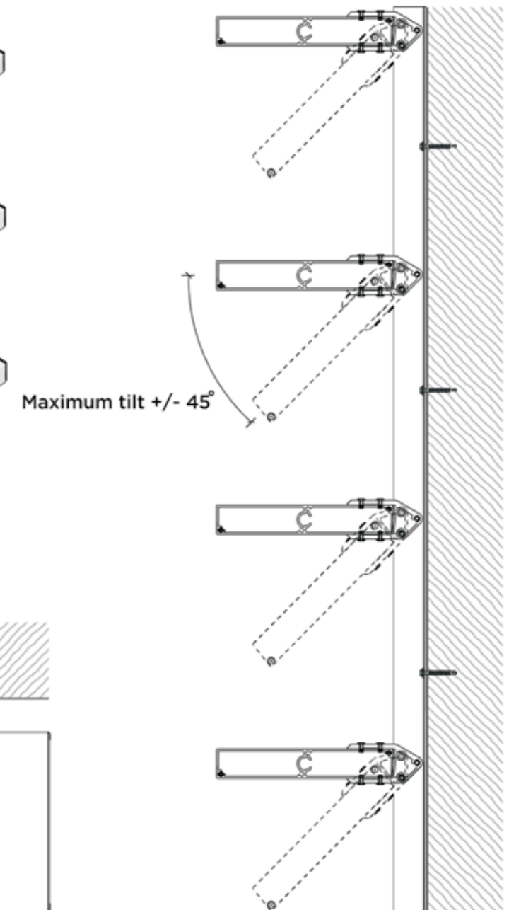
Sectional View
