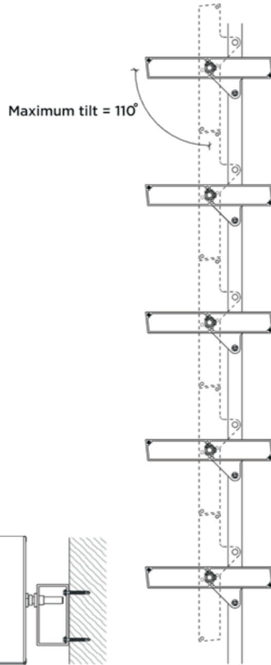
Sectional View
